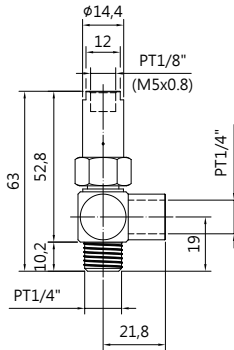
FPC-1/4" (M5 Pilot hole) FPC-1/4"S (1/8" Pilot hole)
